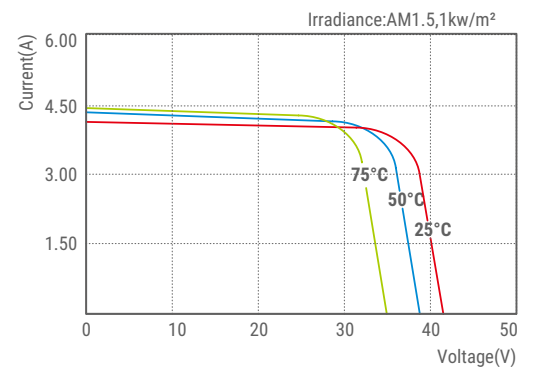
SLP150S-24U I-V Curves
